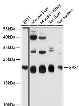
Fig. 1. Western blot analysis of extracts of various cell lines, using GPX1 antibody at 1:1000 dilution. Secondary antibody: HRP-labeled Goat Anti-Rabbit IgG(H+L) (A0208) at 1:1000 dilution. Lysates/proteins: 25µg per lane. Blocking buffer: QuickBlock™ Blocking Buffer (P0231). Detection: BeyoECL Star (P0018A). Exposure time: 1s.
